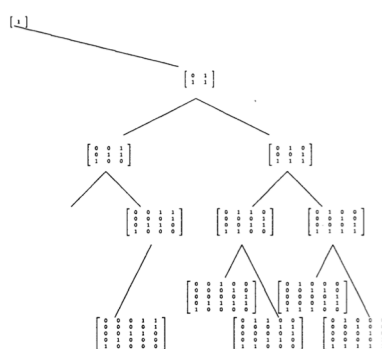
Fig.2 Tree of topological Markov chains, T_n .
